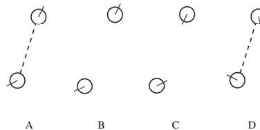
Figure 1: Basic algorithm
